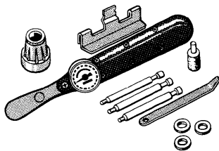
2108268 KIT, DISK REPLACEMENT, 1405 CONSISTING OF 45740 WASHER 3/8 2108027 DISK INSTALLING TOOL 2108040 ADAPTER, SOCKET WRENCH 3/8 SQ DR, 5/16 HEX 2108041 BOLT, 3/8-24, PULLDOWN, SPL. 2108051 TIP, CLUTCH 2108314 CLAMP, DISK POSITIONING 2108570 DISK ALIGNING TOOL
