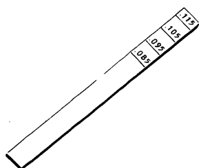
2108576 GAUGE, CARRIAGE SPACING 1301
