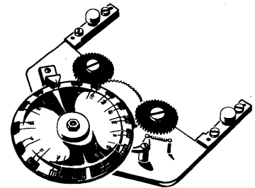
**123635 GAUGE, COUNTER 402-405
