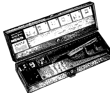
461038 DIE SET, CRIMP, BURNDY N22R VT-1 461121 DIE SET, CRIMP, BURNDY N12RT-3 461122 DIE SET, CRIMP, BURNDY N12ECT 461036 CRIMPING TOOL, HANDLE, BURNDY M8ND
