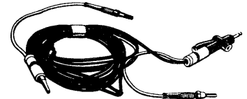
*4261093 SYNC LEAD, SHIELDED 4261081 TEST LEAD, SHIELDED 4261080 COUPLING, BANANA PLUG, 6-32 451659 BANANA TIP, 6-32 461119 TIP, PROBE, 6-32
