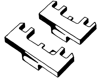
GAUGE, ADDING UNIT 460192 802 460193 803
