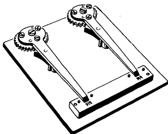
123228 GAUGE, COUNTER SPOOL
